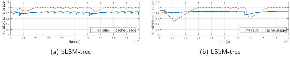
Fig. 13. Hit ratios of tests on Zipfian workloads.
