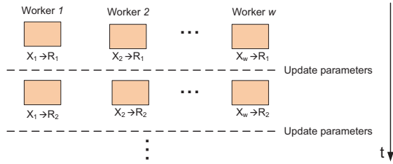
Figure 2. Process of the subrange concurrent method. Each worker recomputes the distribution among the subrange ( R_i ) for all of its local data points ( X_j ).
