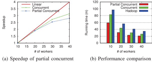
Figure 6. Scaling performance of the partial concurrent method.
