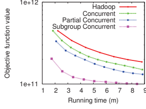
(a) K-means on Covtype
