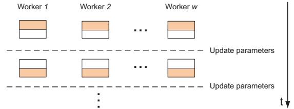
Figure 1. Process of the partial concurrent method. The colored box indicates the picked block of data points for computing the distribution.
