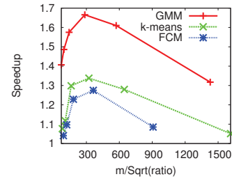
Figure 8. Speedup. X-axis represents the values of m/\sqrt{\frac{T_{vhd}}{T_{sgl}}} .
