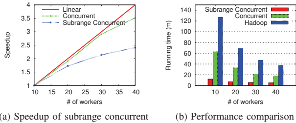
Figure 7. Scaling performance of the subrange concurrent method.
