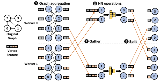
Figure 6: GNN tensor parallelism workflow for a single layer.
